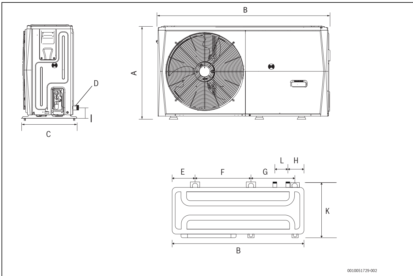
SI.32 Modeli CS2000AWF 4 R-S do CS2000AWF 6 R-S
