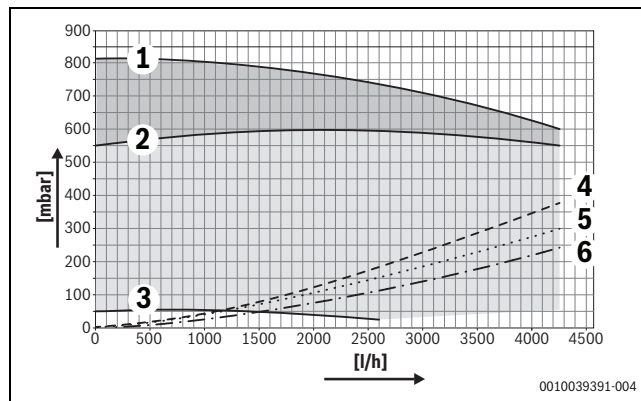
SL.52 Preostala visina isporuke pumpe 85kW-100kW
